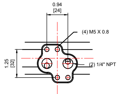
NAMUR 1/4" NPT Air connector
