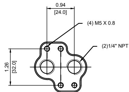
NAMUR 1/4" NPT Air connector
