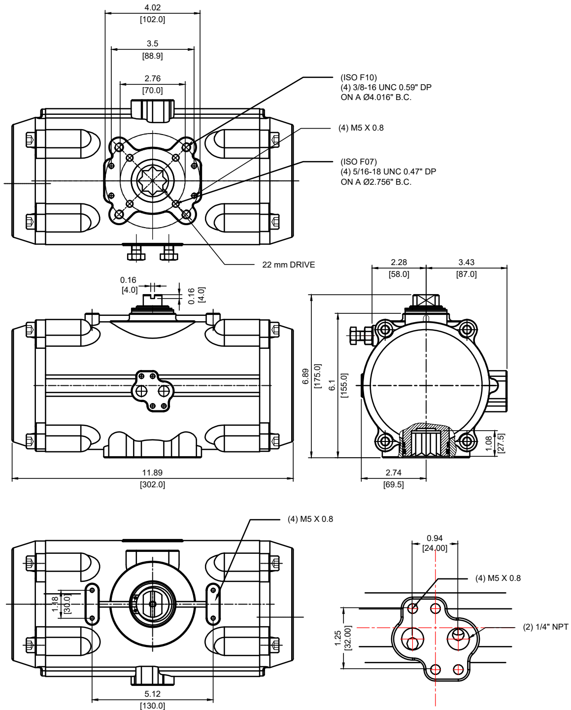
NAMUR 1/4" NPT Air connector
