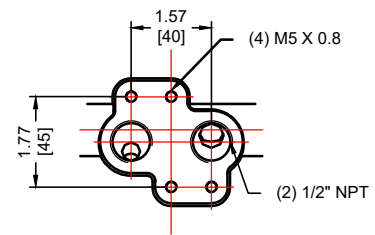
NAMUR 1/2" NPT Air connector
